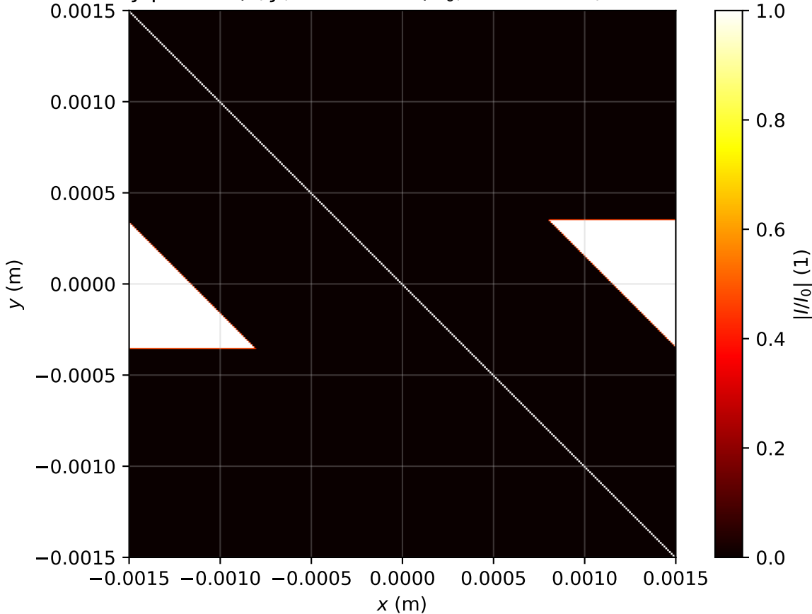
Intensity profile I(x, y, z = 0.000\text{m})/I_0 , \text{Pin}=3.0\text{Pcr} , artificial time
